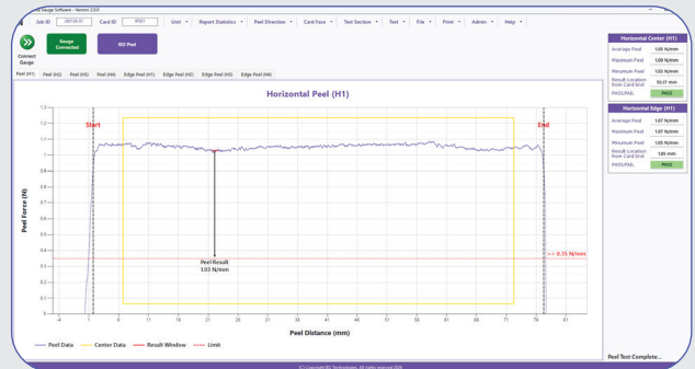
Sample Peel Test Graph
