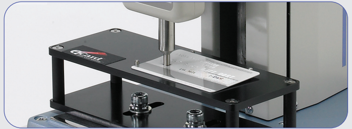
Back of Card Spot Pressure (push test)
