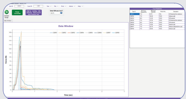
Sample Backside Spot Pressure Graph
