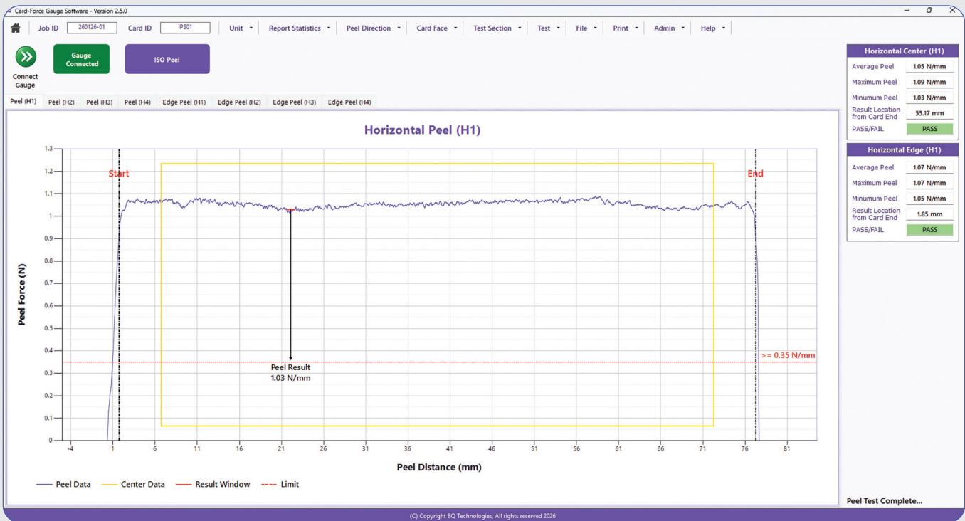
Sample Peel Test Graph
